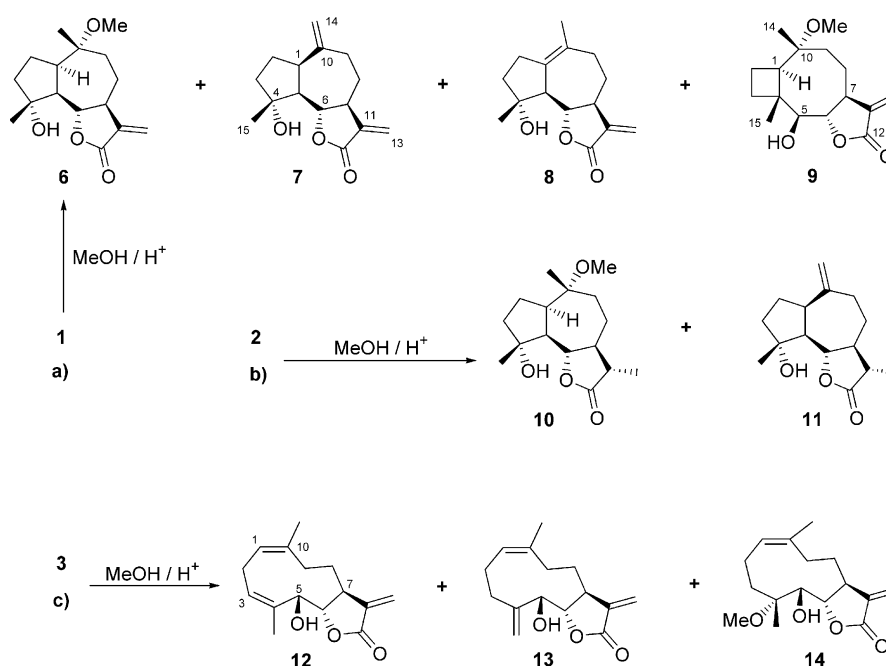
Figure 2. Reactions of 1 , 2 and 3 with pTSA / MeOH.
