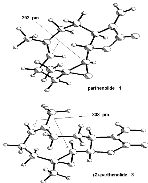
Figure 4. MM-calculated lowest energy conformers of 1 and 3 and their C(1)–C(5) interatomic distances.
