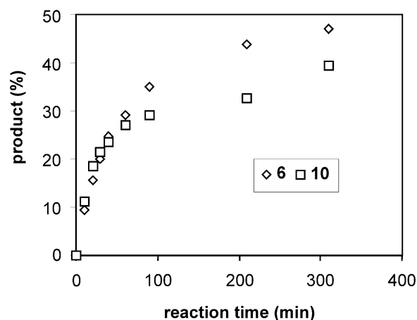
Figure 3. Formation rates of 6 and 10 from acid catalyzed reactions of 1 and 2 (see Experimental).
