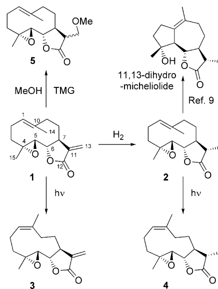
Figure 1. Chemical transformations of 1 .
