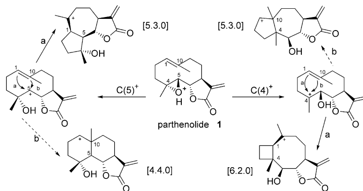
Figure 5. Mechanisms of acid-catalyzed transannular cyclization of 1 . The formation of cation at C(5) is preferred with respect to C(4); the pathways a are exclusively observed whilst the pathways b do not occur. IUPAC notations for bicyclic decane ring systems are reported in square brackets.
